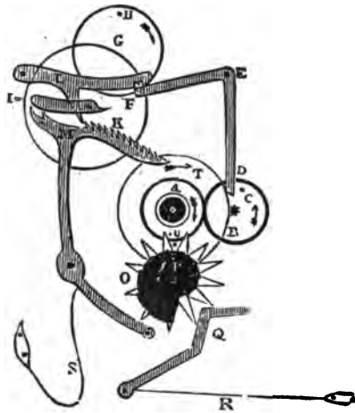
Rack Striking Work.
