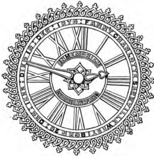
Memorial Turret Clock Dial.
