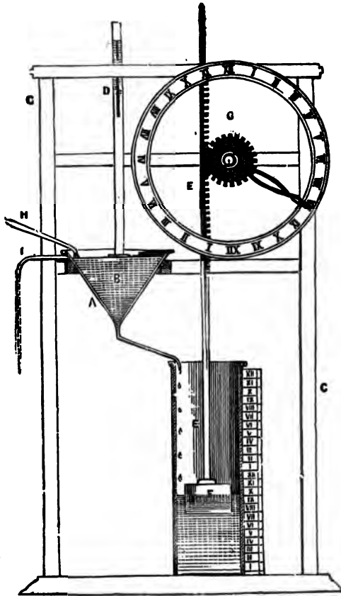
The Clepsydra, or Water-Clock of the Greeks.
