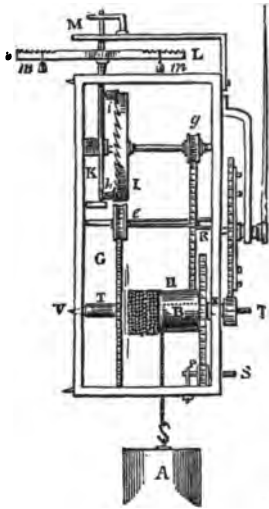
Old Balance Clock.
