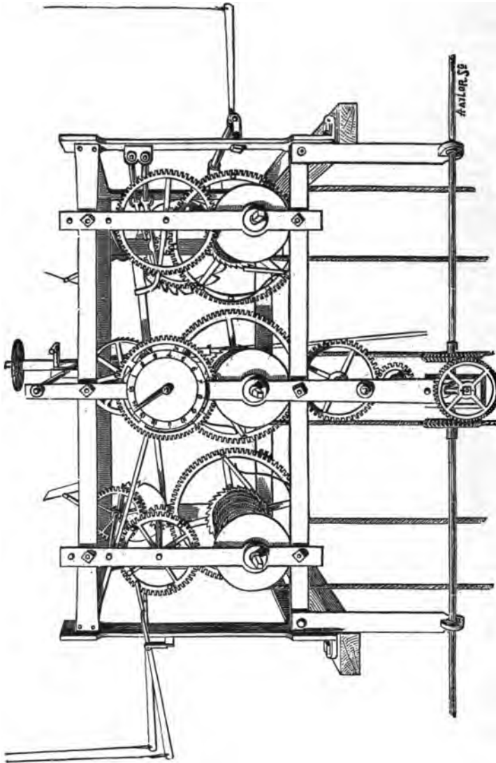
St. James's Palace Clock.
