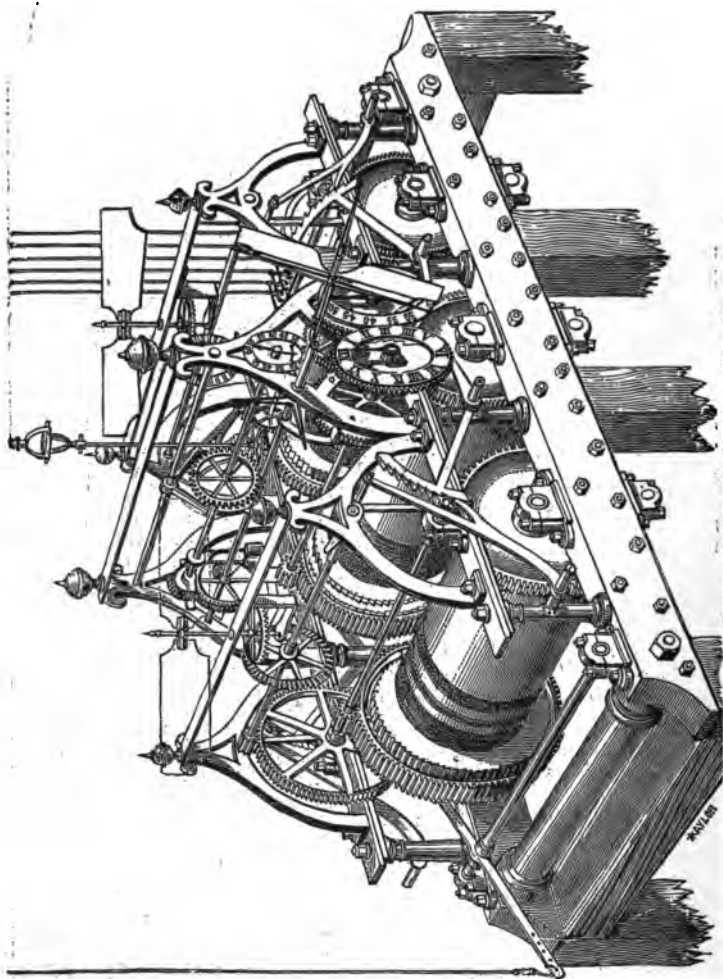
Benson's Great Clock.—The Movement.
