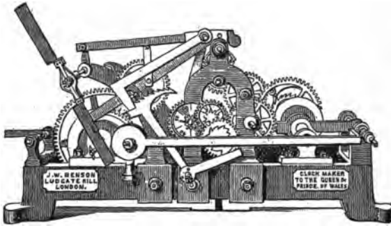
A Modern Turret Clock.
