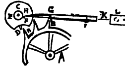
Chronometer Escape- ment.
